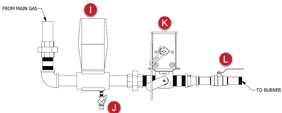
Figure 1. Batch Burn-Off Oven primary gas train components
