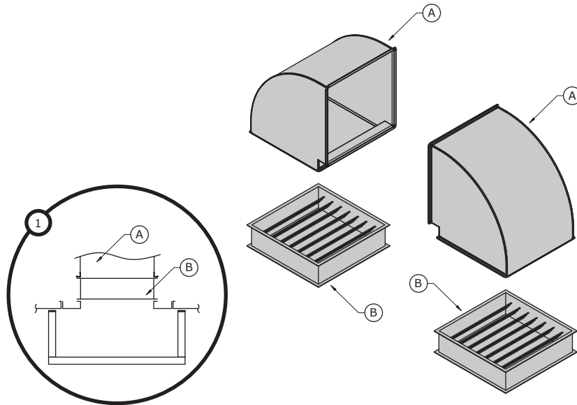
A: AMU B: Damper with sleeve
