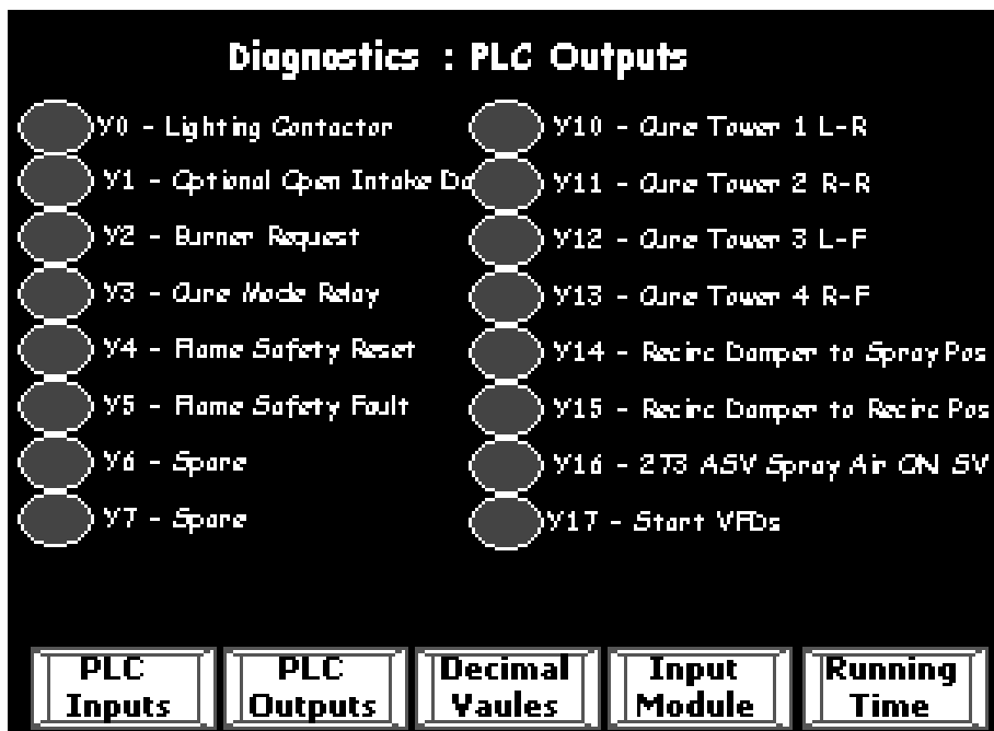
Figure 22. PLC Outputs screen
