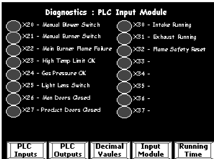
Figure 24. PLC Input Module screen
