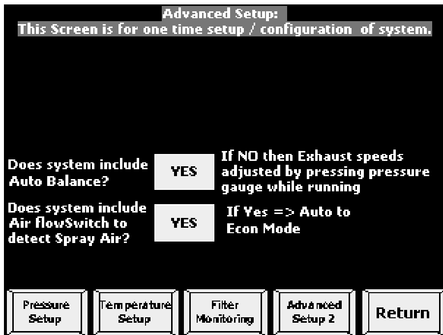
Figure 26. LOGIC 3 Advanced Setup with manual balance
