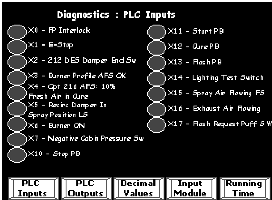
Figure 21. PLC Inputs screen
